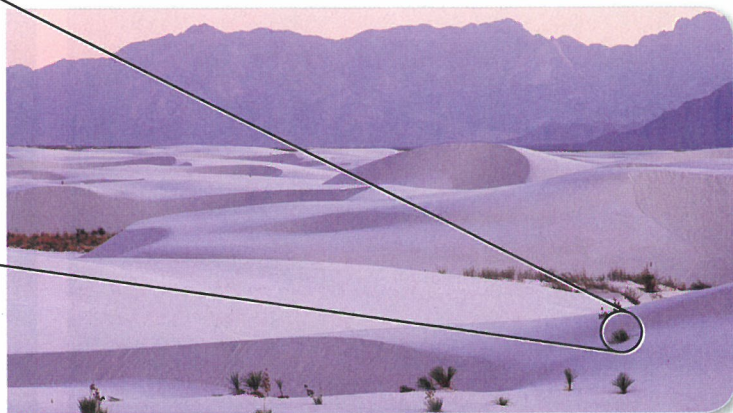
■ Figure 6.3 These sand dunes at White Sands National Monument in New Mexico were formed by wind-blown sand that has been transported and redeposited. Notice the uniform size of the sand grains.
