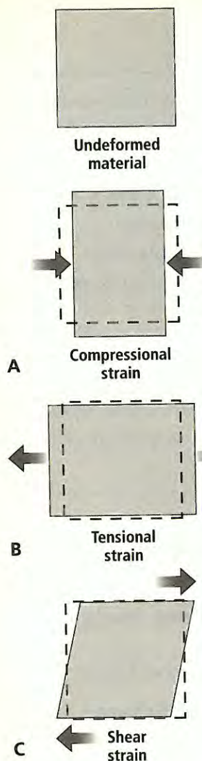
Figure 5-17 Stresses are the forces that act on a material. Strain is the deformation of a material in response to stress. Compressional forces make a material shorter (A). Tensional forces make a material longer (B). Shear forces distort a material (C).
