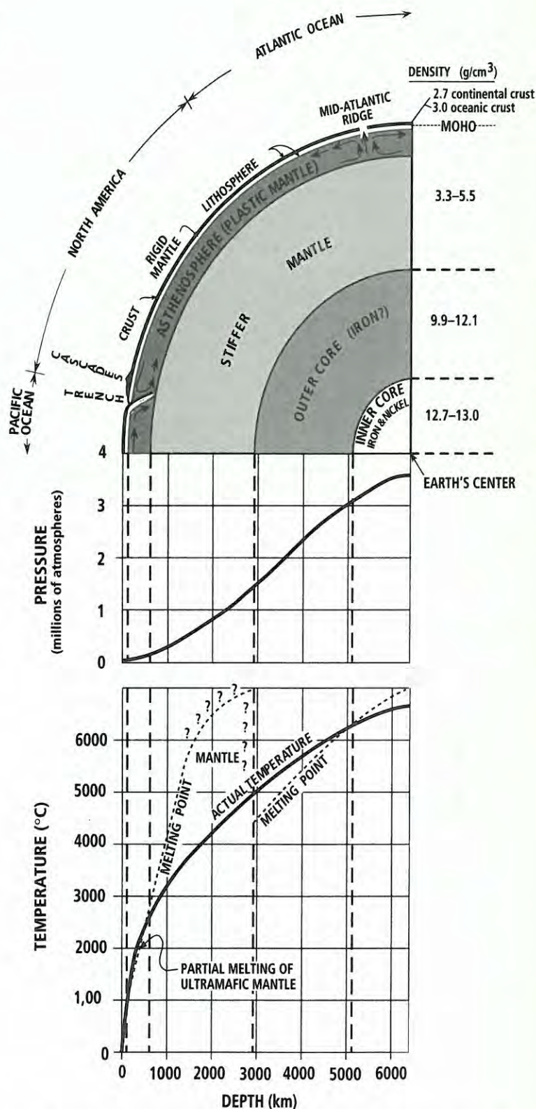
Figure 5-6 Earth's crust and the uppermost part of the mantle form the rigid lithosphere. Beneath the lithosphere is the asthenosphere, the partially molten part of the mantle. Beneath the asthenosphere, a zone of stiffer mantle can be found. Beneath the mantle are the outer core and the inner core, which are composed of mostly iron. The properties of density, pressure, and temperature vary throughout Earth's layers.
