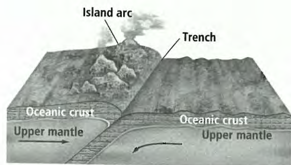
Oceanic-oceanic
