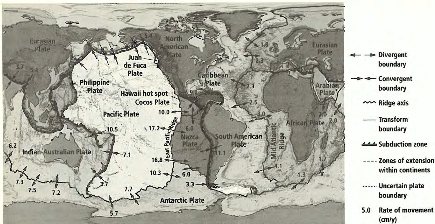
Figure 5-7 Earth's lithosphere is broken into enormous slabs called plates. These plates move slowly over Earth's surface. At divergent boundaries, plates move apart; at convergent boundaries, plates move toward each other; and at transform boundaries, plates move horizontally past each other.
