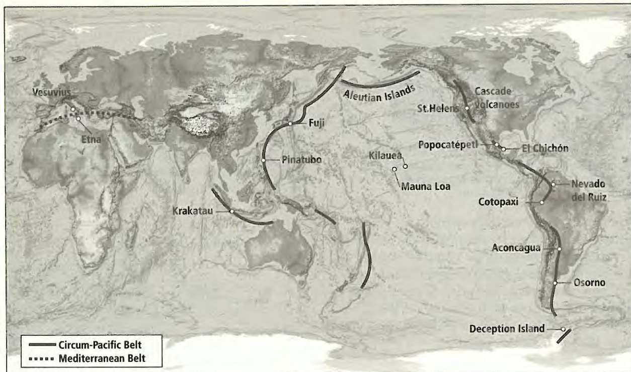
Figure 5-16 Most volcanism on Earth is associated with convergent and divergent plate boundaries. Only about 5 percent of Earth's volcanoes form far from plate boundaries.
