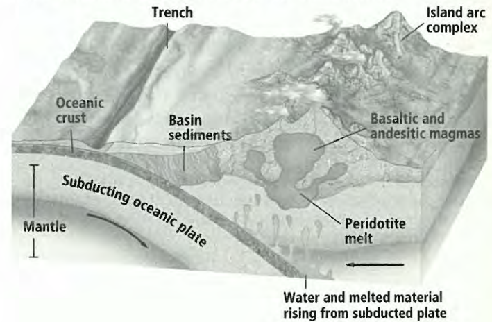
Figure 5-34 Orogeny that involves two oceanic plates forms an oceanic trench, an island arc complex, and a forearc basin that fills with sediments eroded from the islands.
