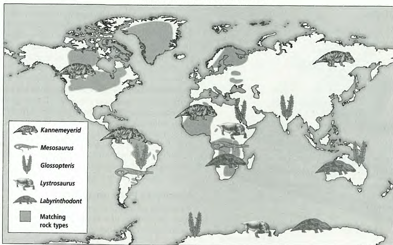
Figure 5-2 Various fossils and the similarity of rock formations on opposite sides of the Atlantic Ocean provide evidence that Earth's continents were once joined.
