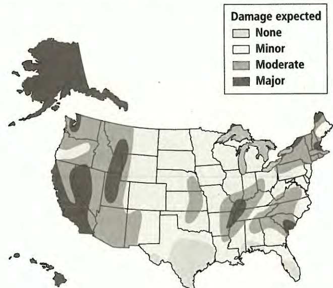
Figure 5-29 Alaska, Hawaii, and parts of other states are areas of high seismic risk.
