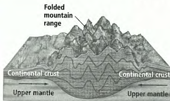
Continental-continental
