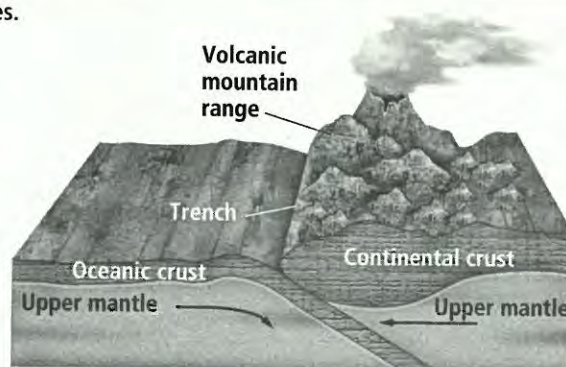
Oceanic-continental
