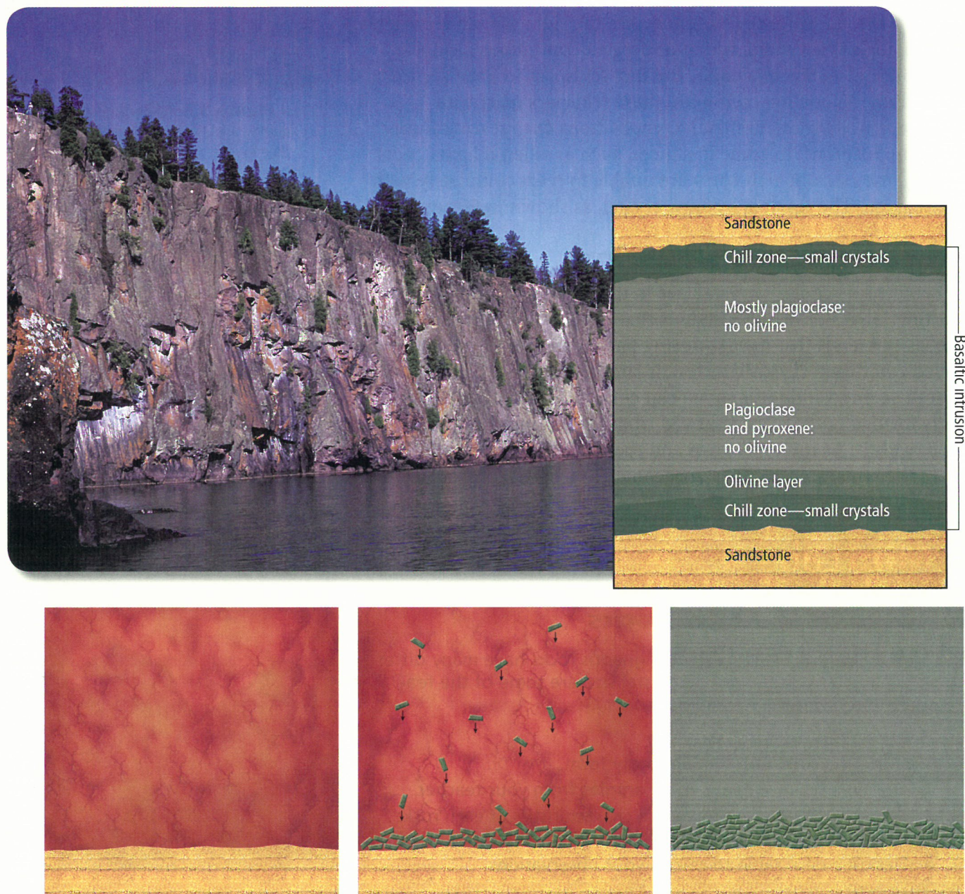
Figure 5.6 The Palisades Sill in the Hudson River valley of New York and New Jersey is a classic example of fractional crystallization and crystal settling. In the basaltic intrusion, small crystals formed in the chill zone as the outer areas of the intrusion cooled more quickly than the interior.
