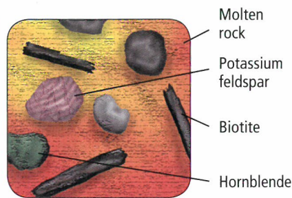
Partially melted rock
